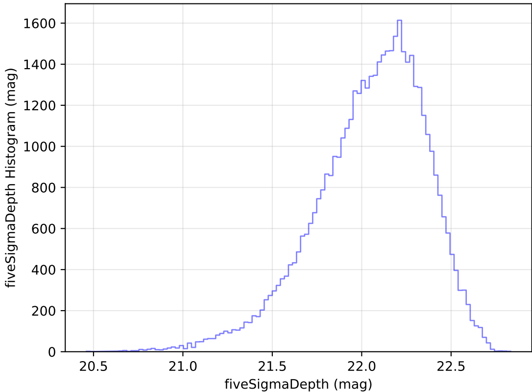
baseline_v3.3_10yrs Yr 1 y band: fiveSigmaDepth Histogram
