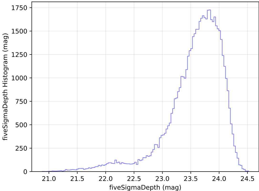
baseline_v3.3_10yrs Yr 1 i band: fiveSigmaDepth Histogram
