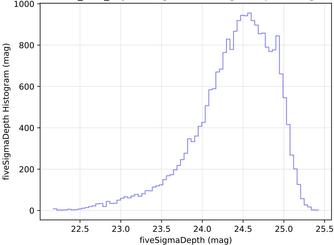
baseline_v3.3_10yrs Yr 1 g band: fiveSigmaDepth Histogram
