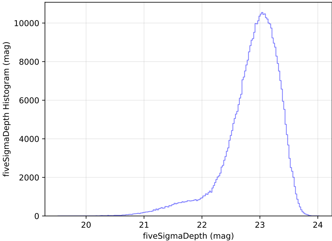
baseline_v3.3_10yrs WFD z band: fiveSigmaDepth Histogram
