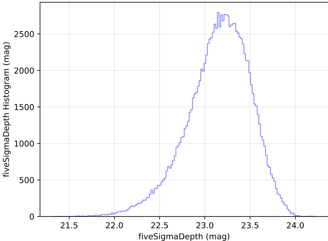
baseline_v3.3_10yrs WFD u band: fiveSigmaDepth Histogram
