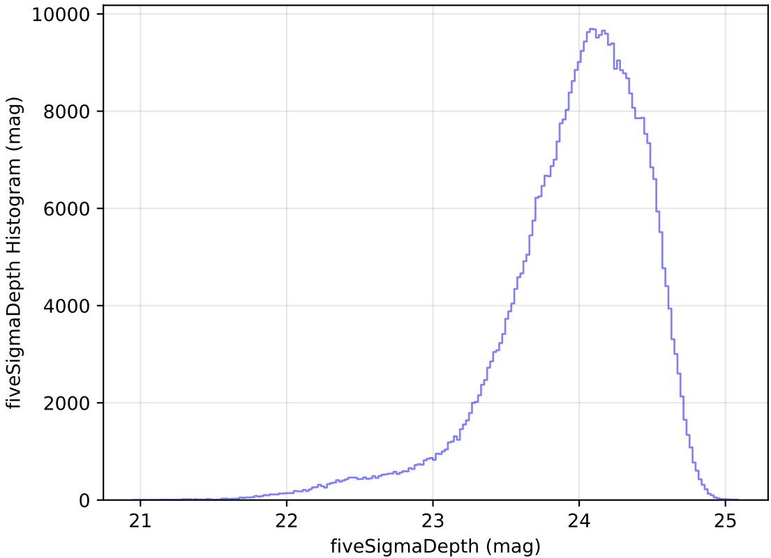
baseline_v3.3_10yrs WFD r band: fiveSigmaDepth Histogram
