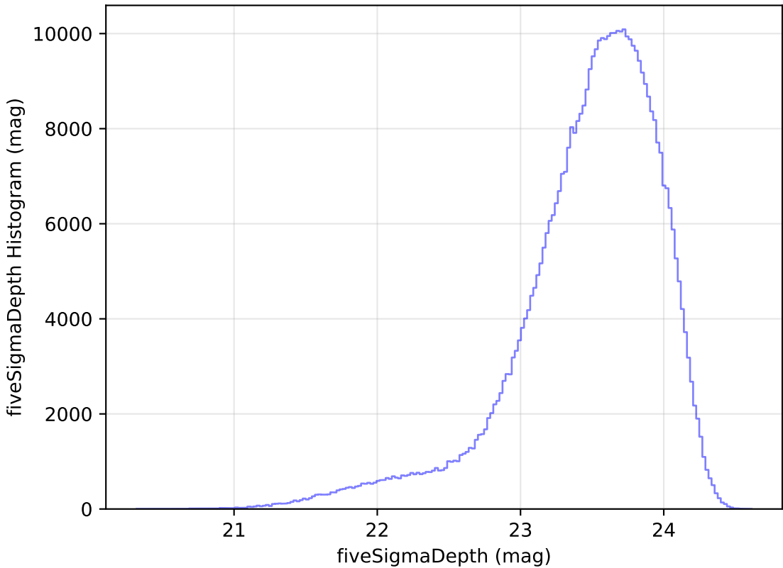
baseline_v3.3_10yrs WFD i band: fiveSigmaDepth Histogram
