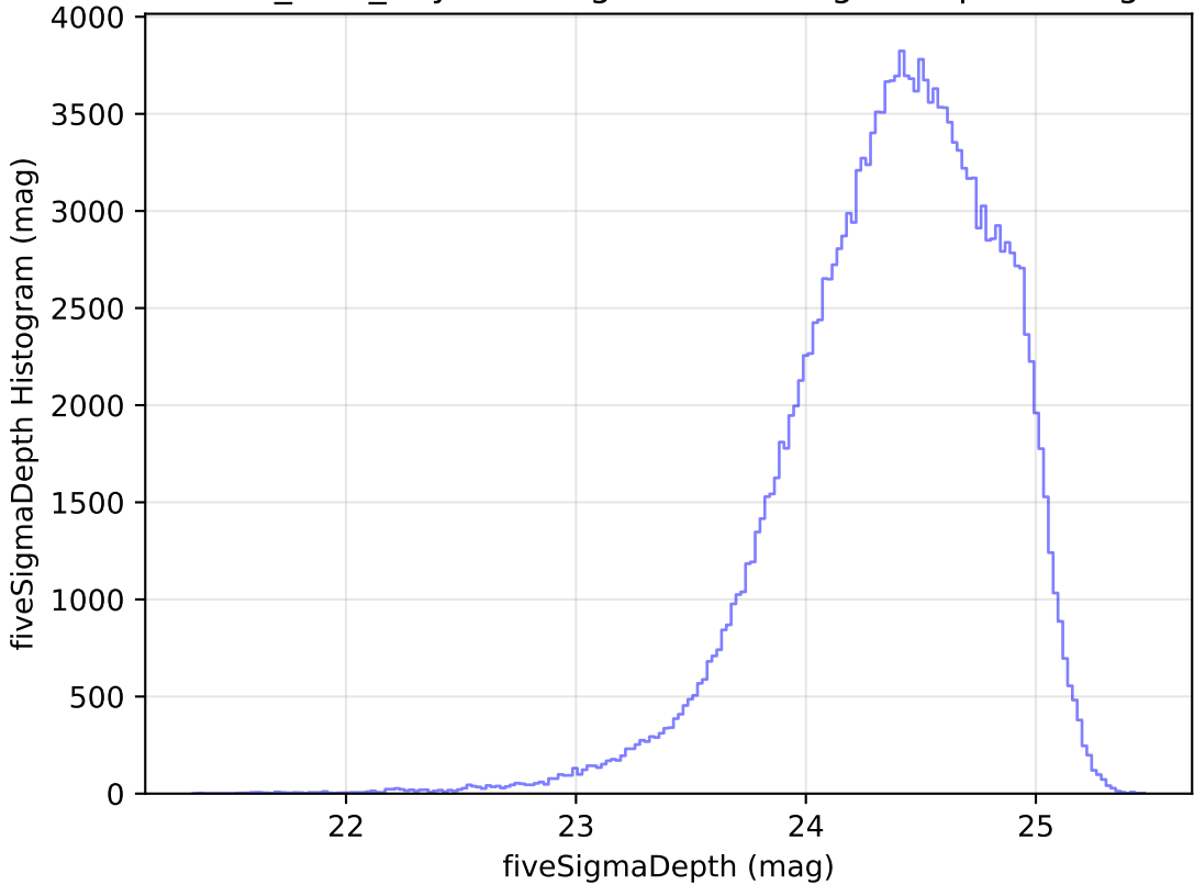
baseline_v3.3_10yrs WFD g band: fiveSigmaDepth Histogram
