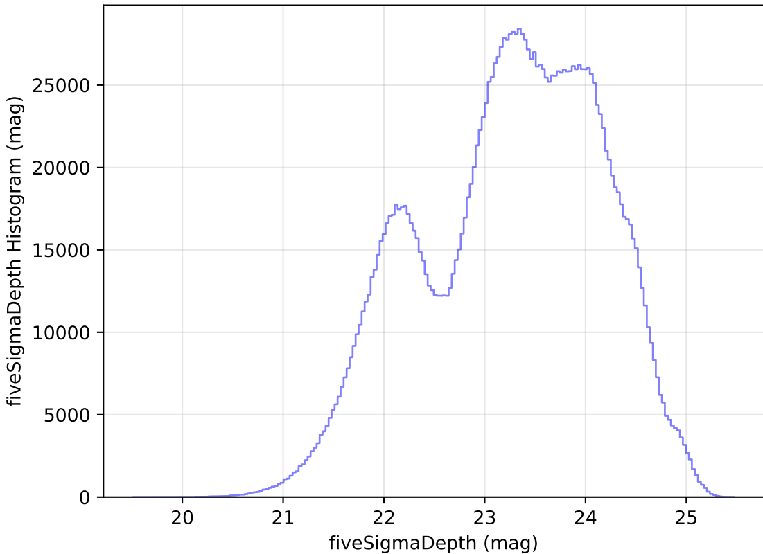
baseline_v3.3_10yrs WFD all bands: fiveSigmaDepth Histogram
