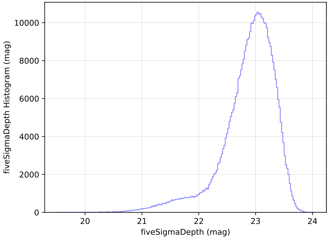
baseline_v3.3_10yrs All sky z band: fiveSigmaDepth Histogram
