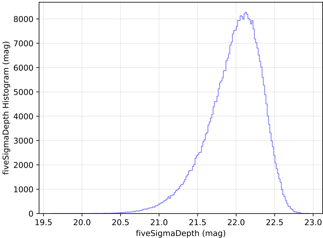
baseline_v3.3_10yrs All sky y band: fiveSigmaDepth Histogram
