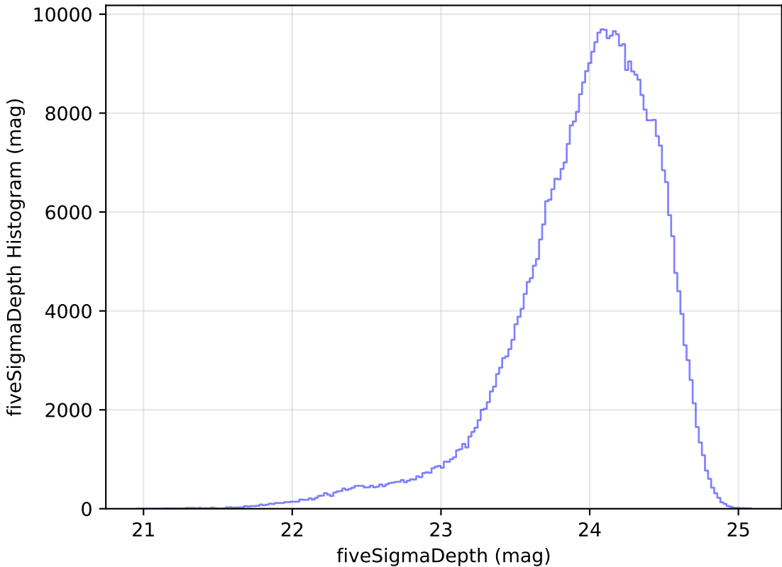
baseline_v3.3_10yrs All sky r band: fiveSigmaDepth Histogram
