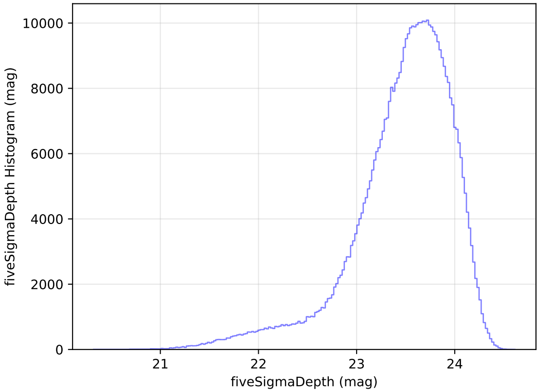
baseline_v3.3_10yrs All sky i band: fiveSigmaDepth Histogram
