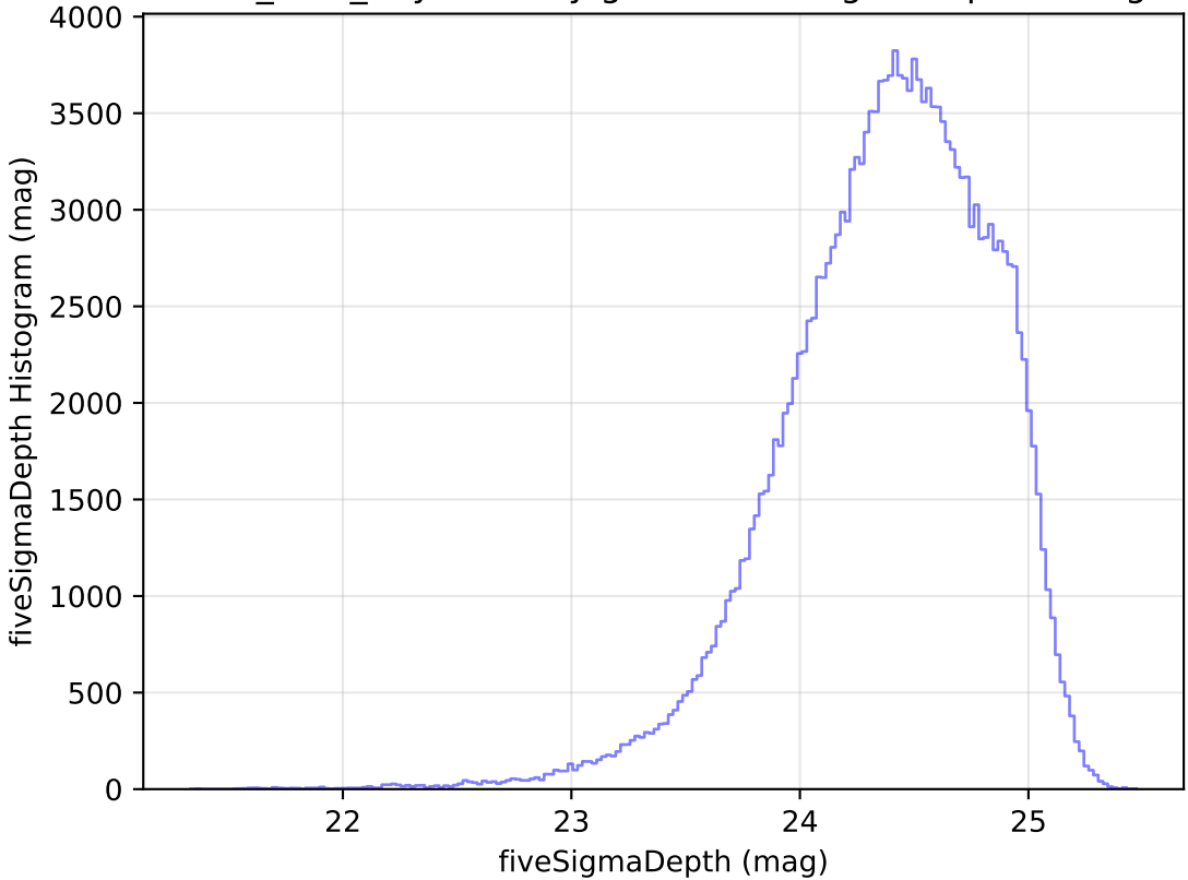
baseline_v3.3_10yrs All sky g band: fiveSigmaDepth Histogram
