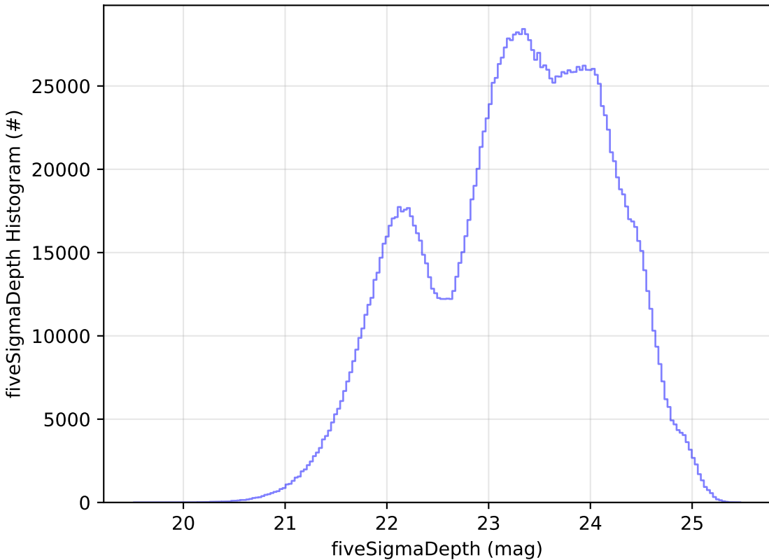
baseline_v3.3_10yrs All sky all bands: fiveSigmaDepth Histogram
