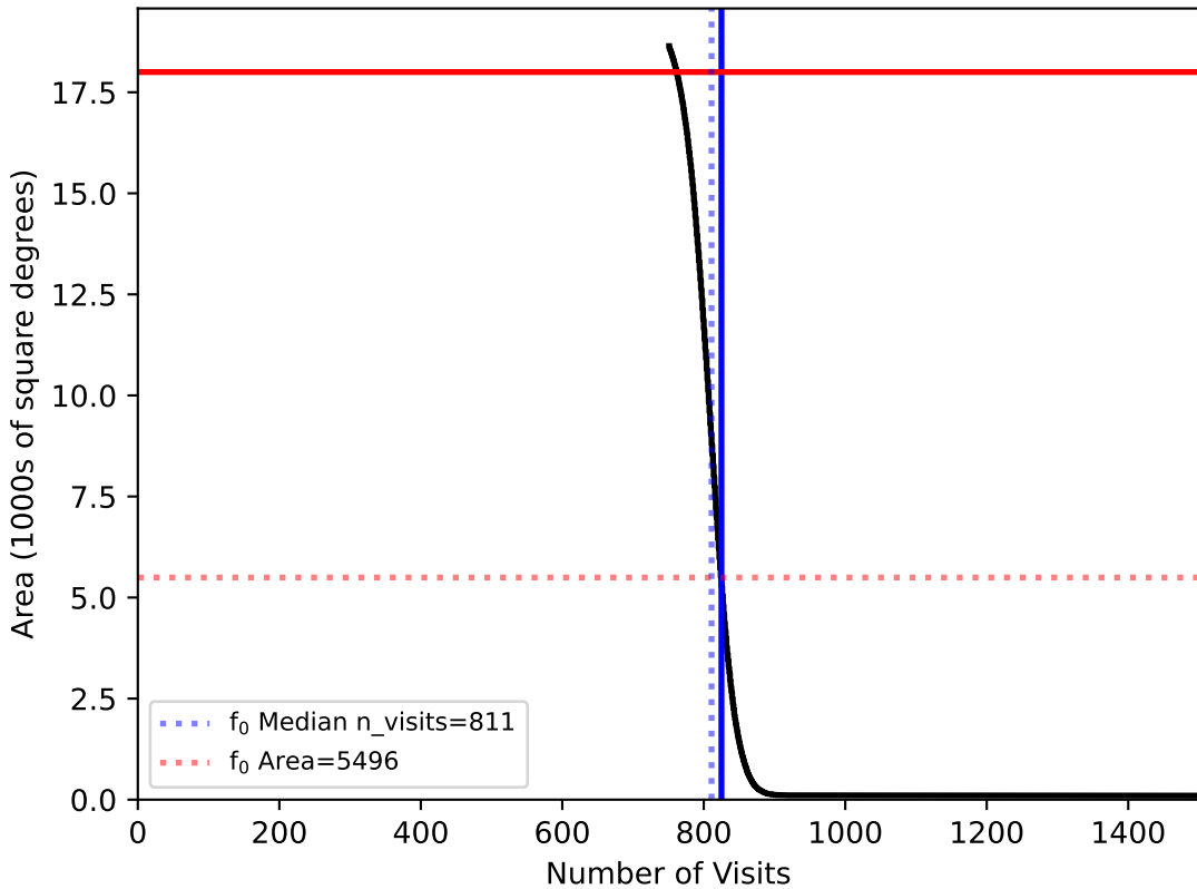
baseline_v3.3_10yrs WFD: f0
