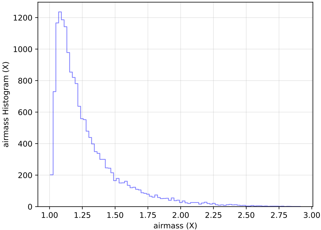
baseline_v3.3_10yrs Yr 1 u band: airmass Histogram
