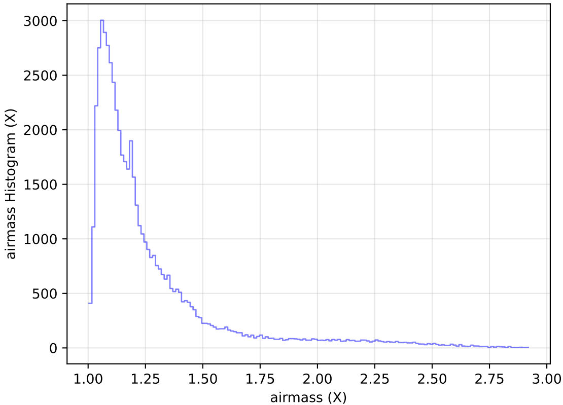
baseline_v3.3_10yrs Yr 1 i band: airmass Histogram
