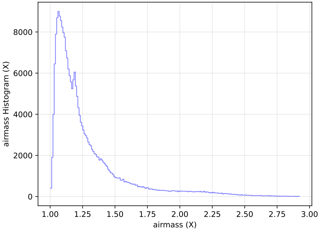
baseline_v3.3_10yrs Yr 1 all bands: airmass Histogram
