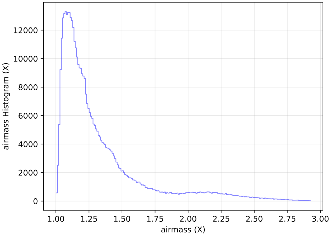
baseline_v3.3_10yrs WFD z band: airmass Histogram
