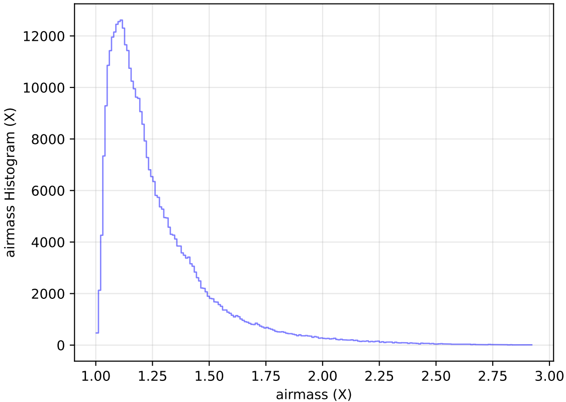
baseline_v3.3_10yrs WFD y band: airmass Histogram
