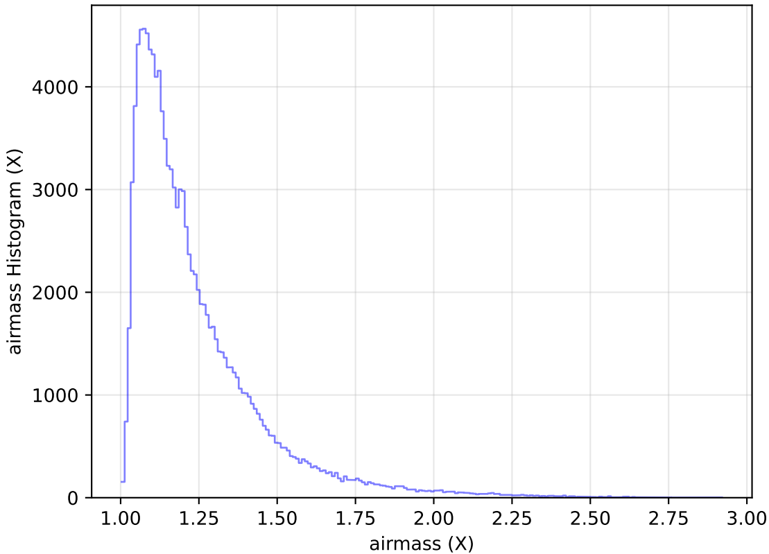
baseline_v3.3_10yrs WFD u band: airmass Histogram
