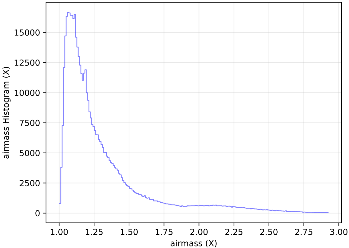
baseline_v3.3_10yrs WFD i band: airmass Histogram
