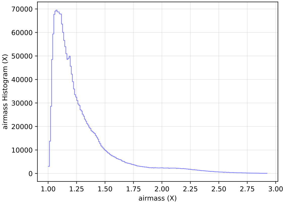
baseline_v3.3_10yrs WFD all bands: airmass Histogram
