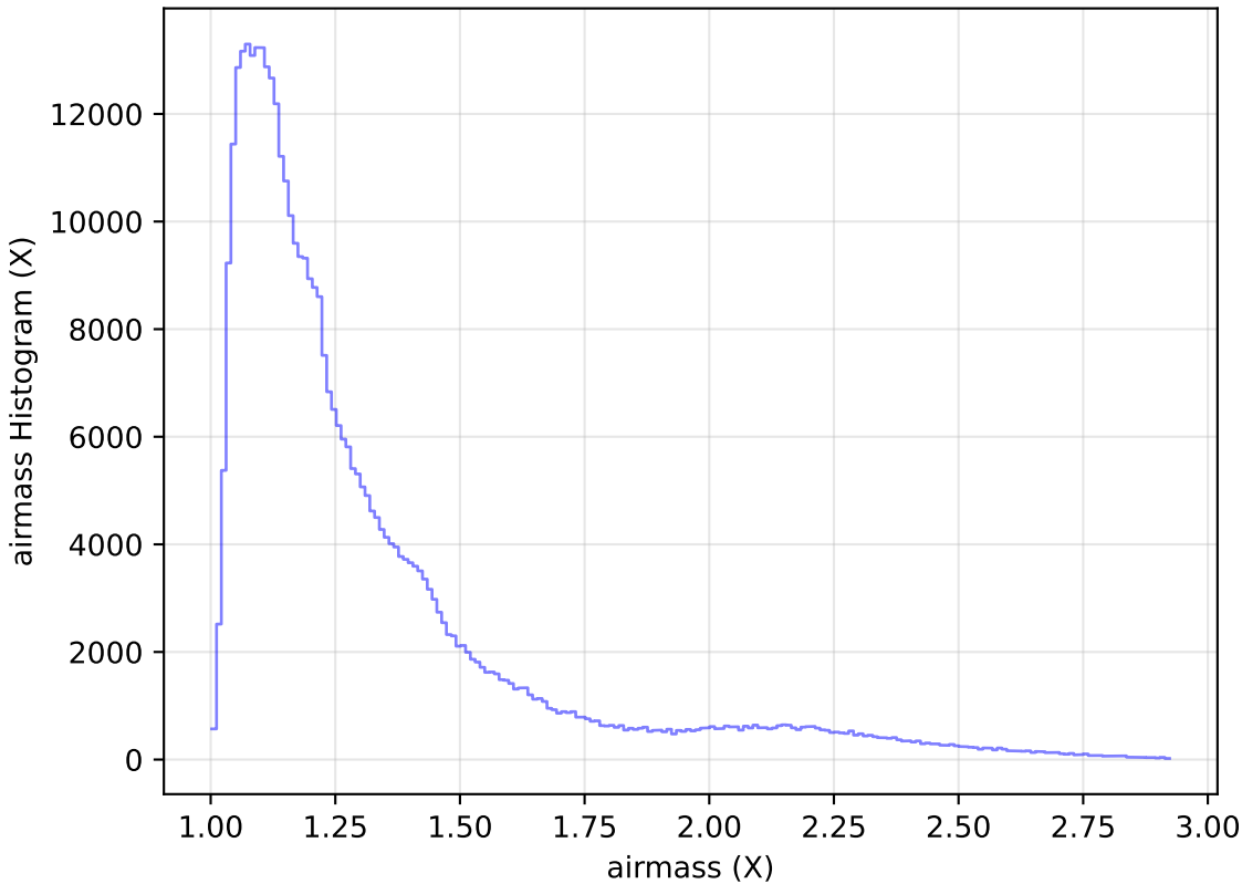
baseline_v3.3_10yrs All sky z band: airmass Histogram
