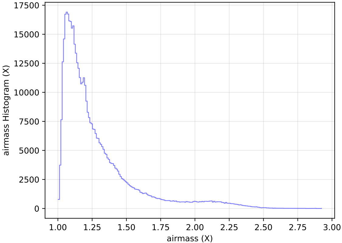
baseline_v3.3_10yrs All sky r band: airmass Histogram
