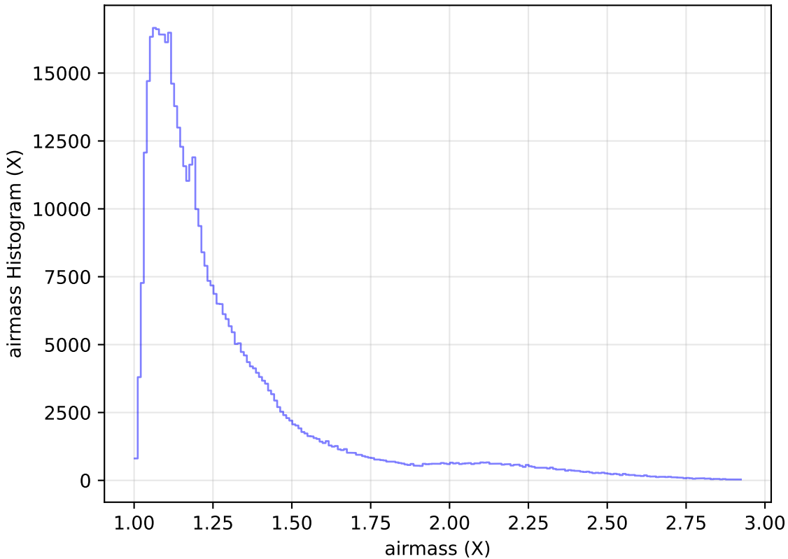
baseline_v3.3_10yrs All sky i band: airmass Histogram
