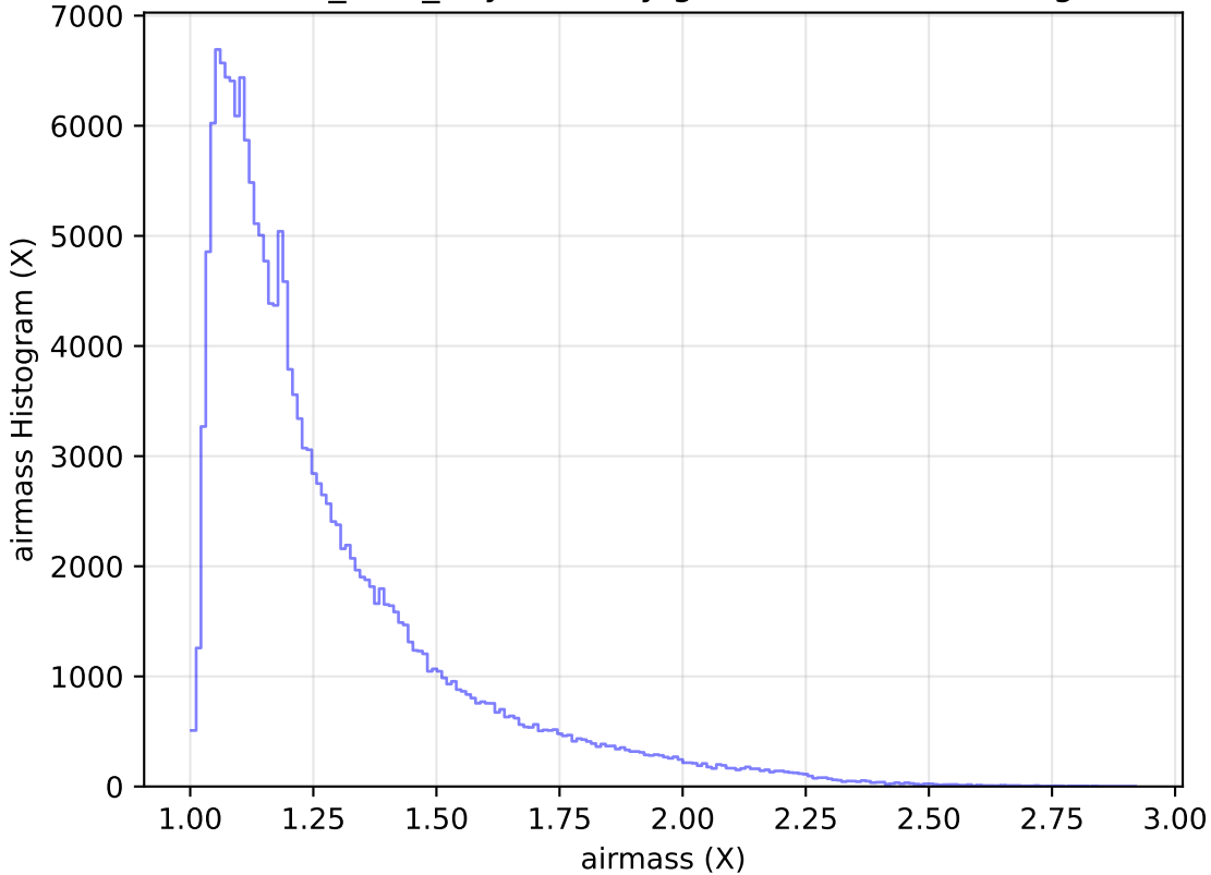
baseline_v3.3_10yrs All sky g band: airmass Histogram
