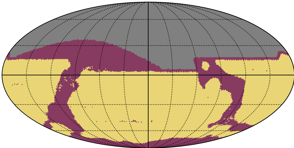
baseline_v3.3_10yrs All sky: RapidRevisits
