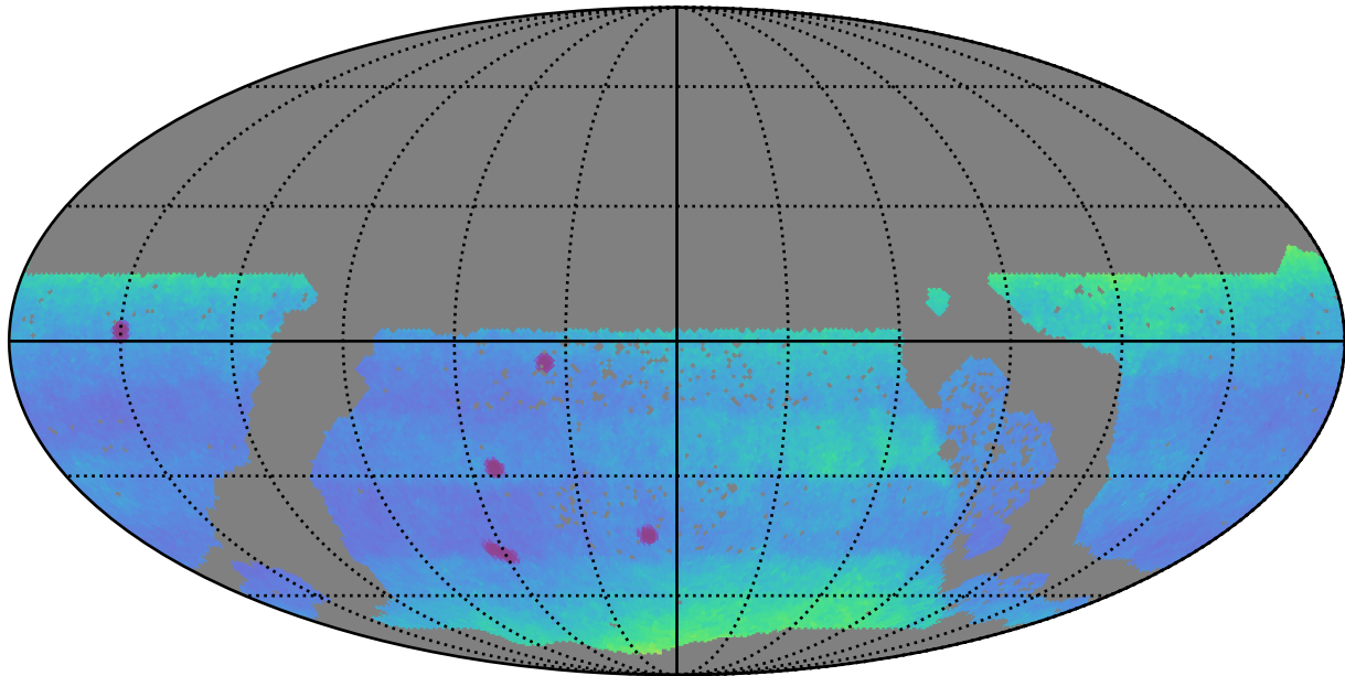
baseline_v3.3_10yrs WFD: Proper Motion Uncert @ 24.0
