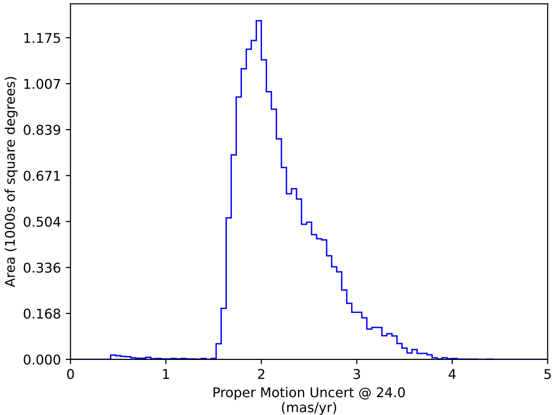
baseline_v3.3_10yrs WFD: Proper Motion Uncert @ 24.0
