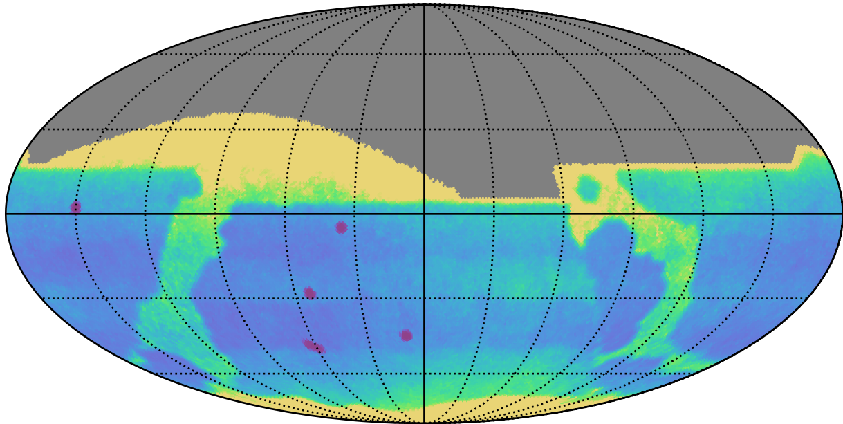
baseline_v3.3_10yrs All sky: Proper Motion Uncert @ 24.0
