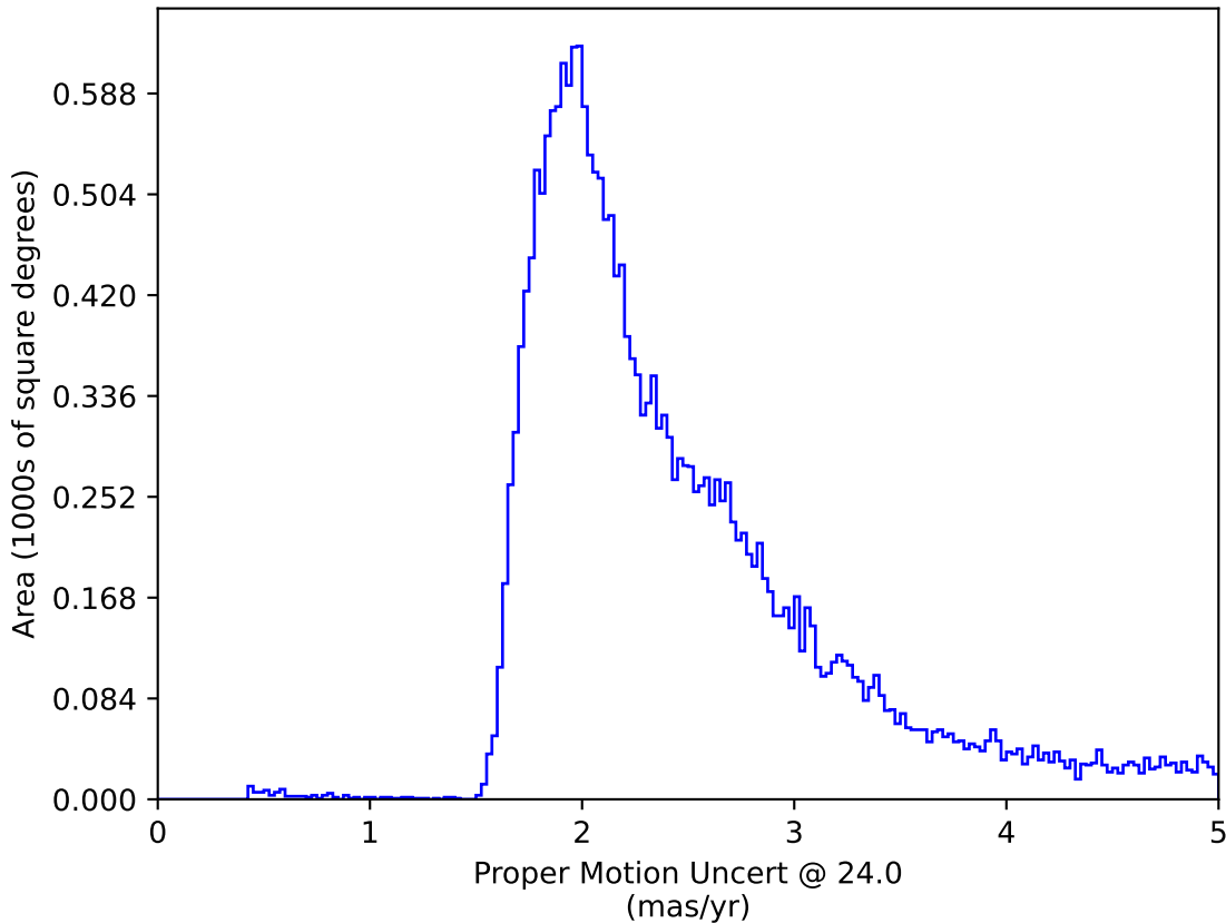
baseline_v3.3_10yrs All sky: Proper Motion Uncert @ 24.0
