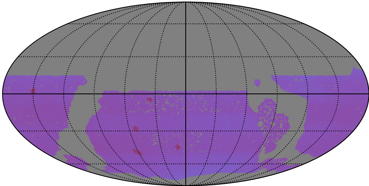
baseline_v3.3_10yrs WFD: Proper Motion Uncert @ 20.5
