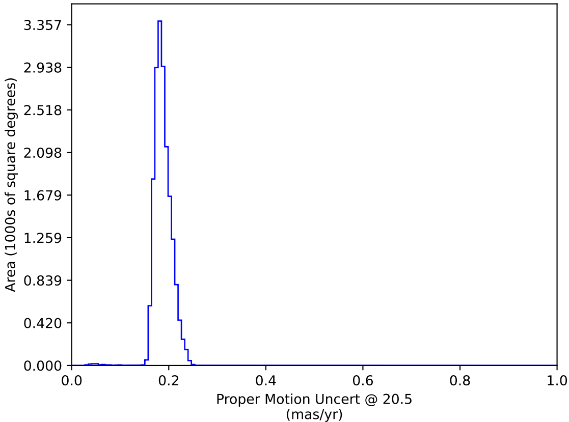
baseline_v3.3_10yrs WFD: Proper Motion Uncert @ 20.5
