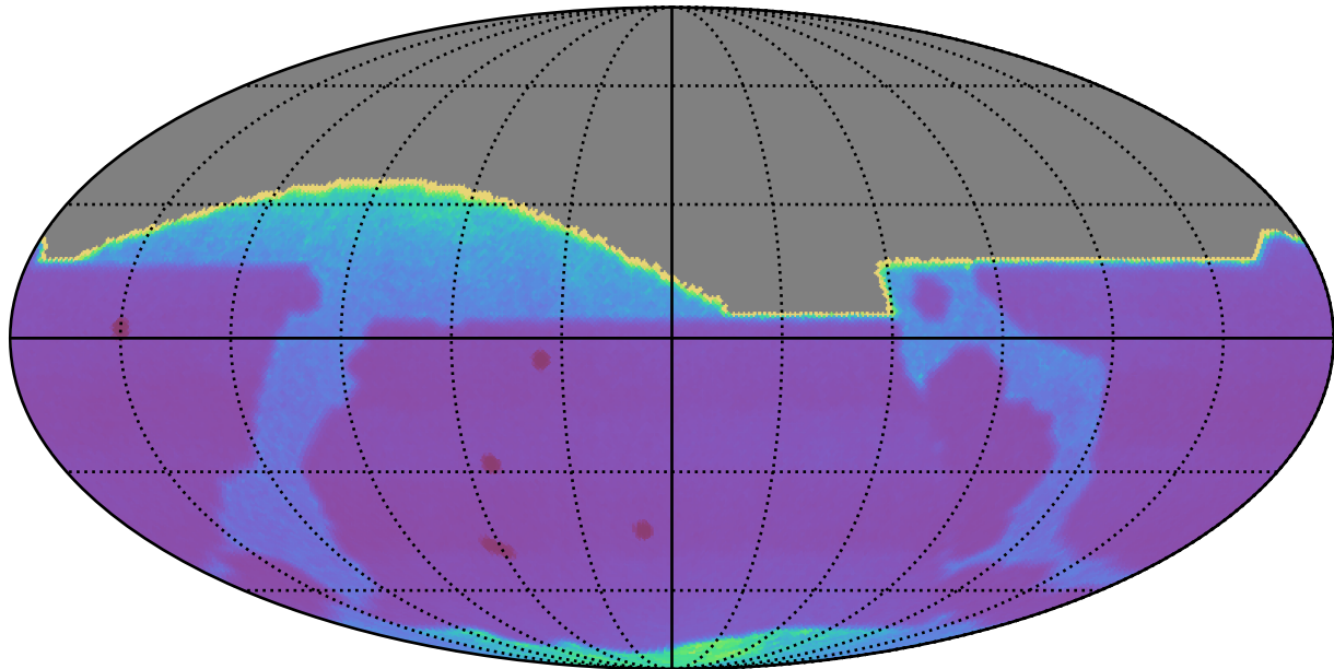
baseline_v3.3_10yrs All sky: Proper Motion Uncert @ 20.5
