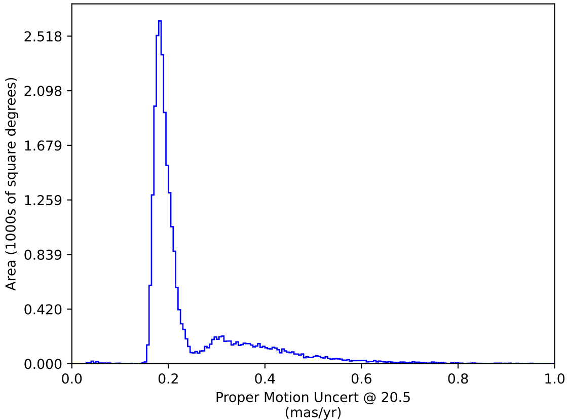
baseline_v3.3_10yrs All sky: Proper Motion Uncert @ 20.5
