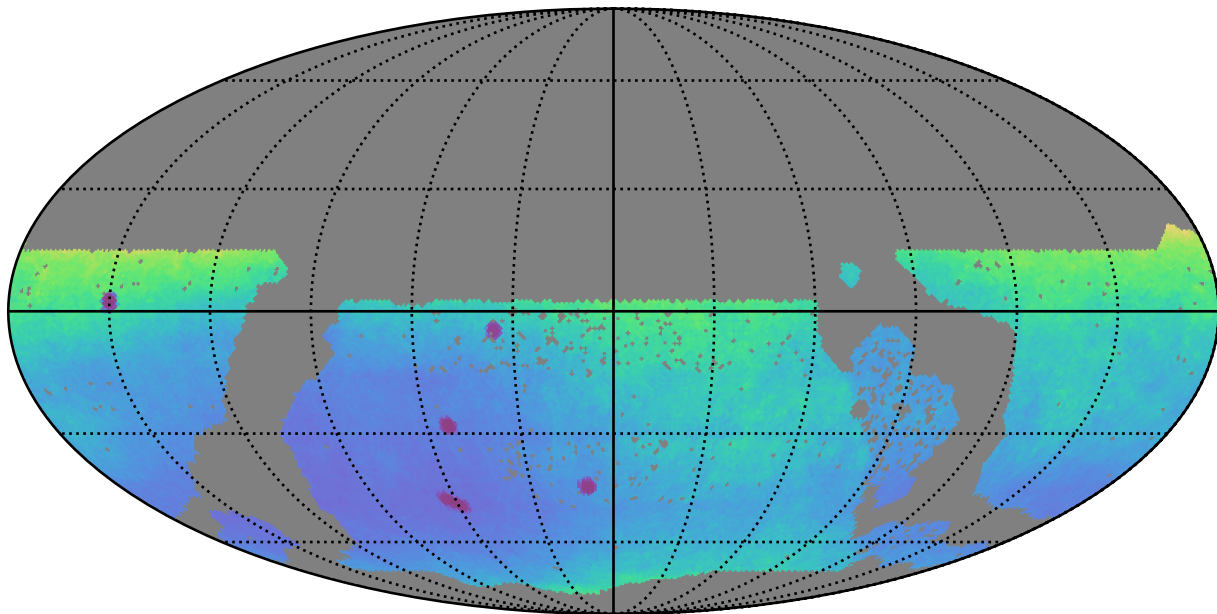
baseline_v3.3_10yrs WFD: Parallax Uncert @ 24.0
