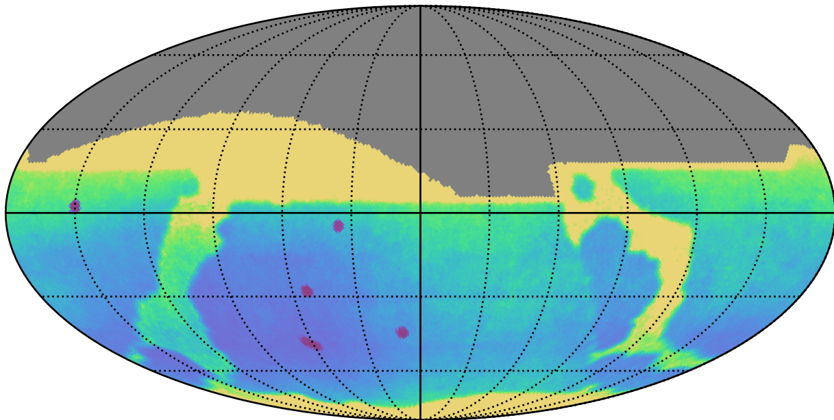
baseline_v3.3_10yrs All sky: Parallax Uncert @ 24.0
