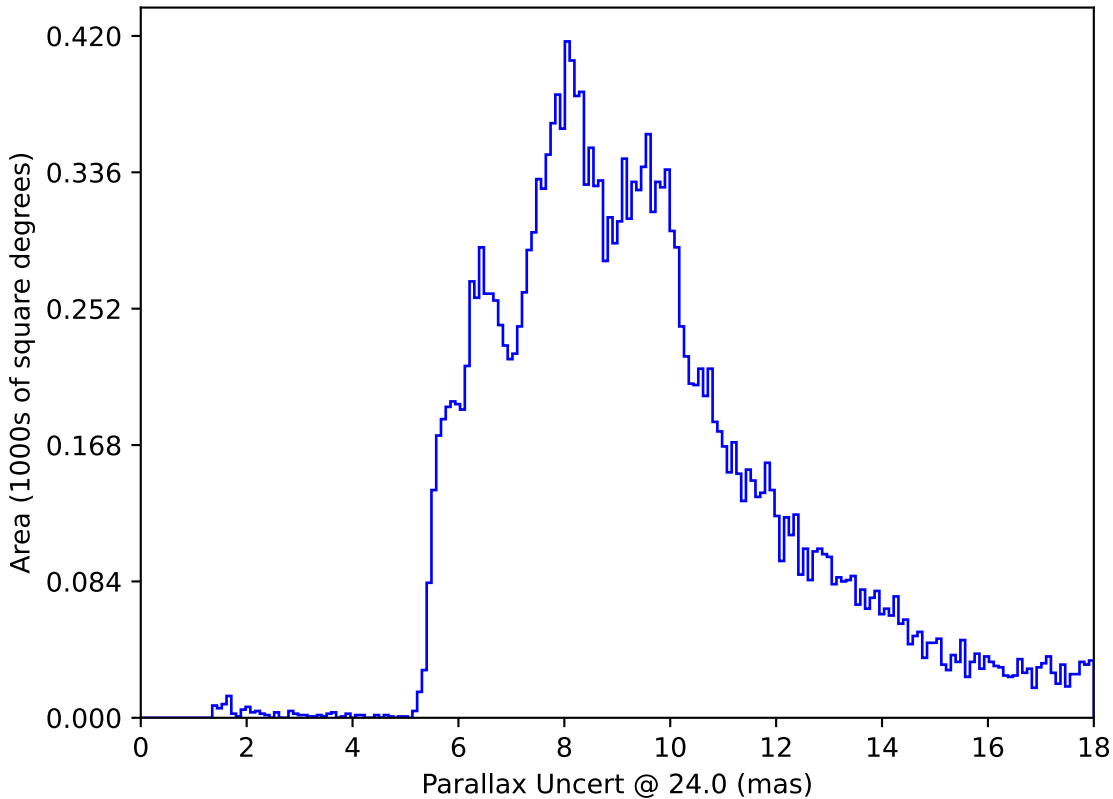
baseline_v3.3_10yrs All sky: Parallax Uncert @ 24.0
