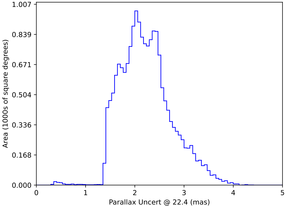
baseline_v3.3_10yrs WFD: Parallax Uncert @ 22.4
