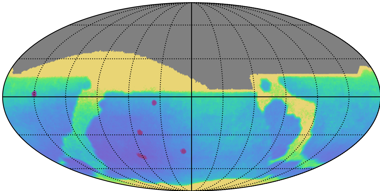
baseline_v3.3_10yrs All sky: Parallax Uncert @ 22.4
