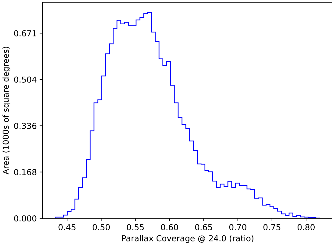
baseline_v3.3_10yrs WFD: Parallax Coverage @ 24.0
