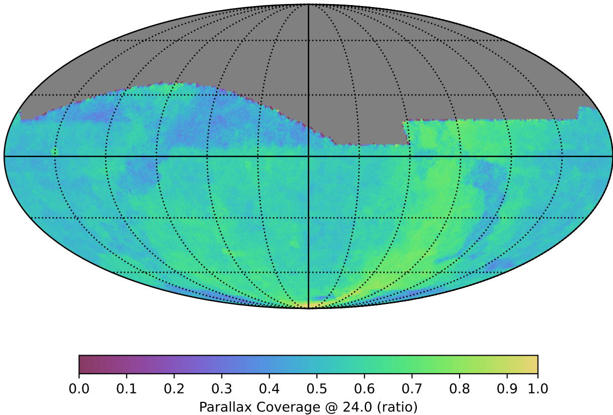
baseline_v3.3_10yrs All sky: Parallax Coverage @ 24.0
