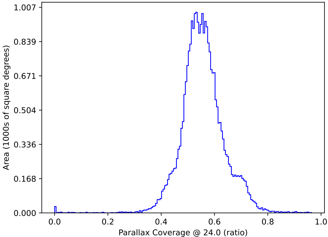
baseline_v3.3_10yrs All sky: Parallax Coverage @ 24.0
