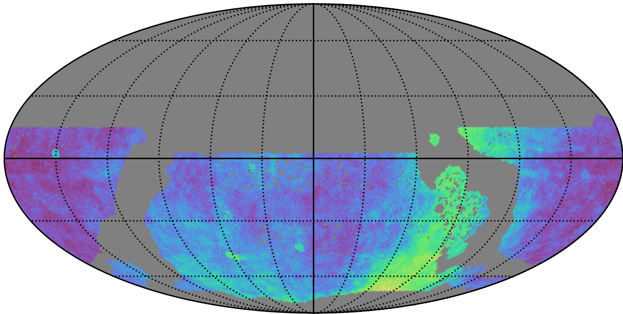
baseline_v3.3_10yrs WFD: Parallax Coverage @ 22.4
