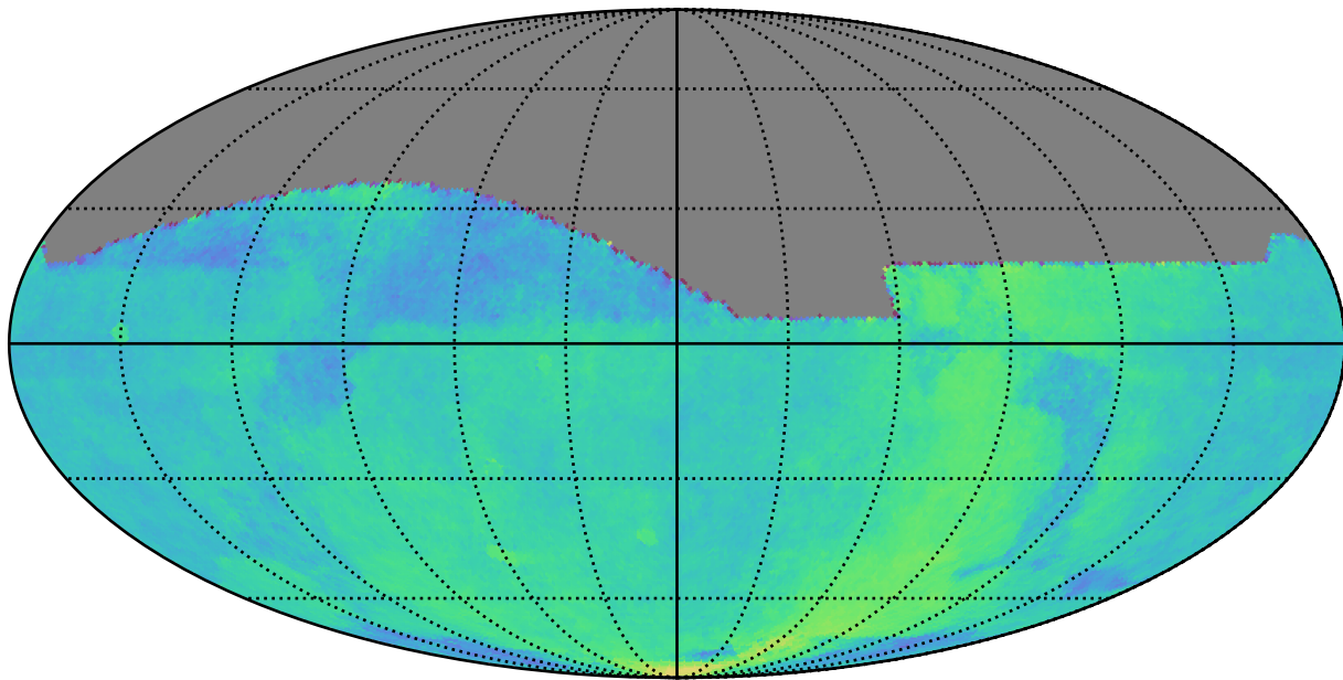
baseline_v3.3_10yrs All sky: Parallax Coverage @ 22.4
