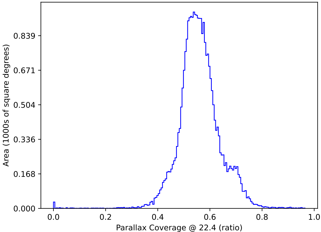
baseline_v3.3_10yrs All sky: Parallax Coverage @ 22.4
