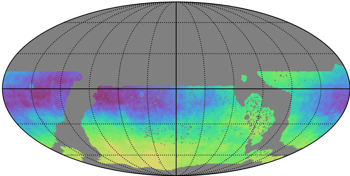
baseline_v3.3_10yrs WFD: Parallax-DCR degeneracy @ 24.0
