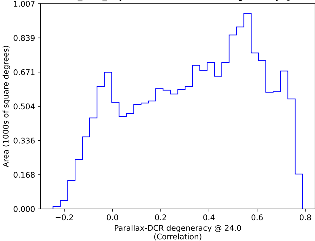
baseline_v3.3_10yrs WFD: Parallax-DCR degeneracy @ 24.0
